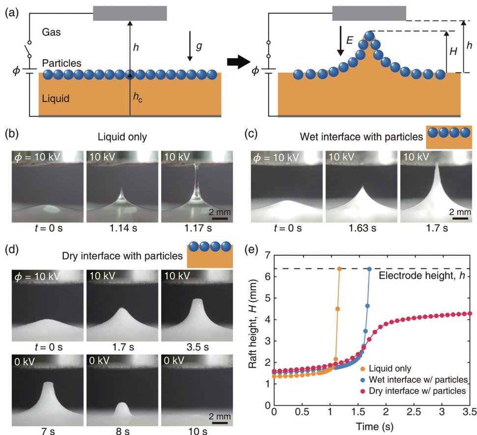
Fig. 1 Electrostatically induced deformation of interfaces. (a) Schematic of the experimental setup. (b and c) A castor oil (b) and a raft of fully wet hollow glass spheres on castor oil (c) develop jets under a strong electric field perpendicular to the unperturbed interface. (d) A raft of partially wet hollow glass spheres on castor oil is upheaved to an equilibrium height without instability, such as ejection, detachment, and interfacial jetting. The upheaved raft due to a high electric potential ( \phi ) descends when the potential is removed, to finally return to a flat interface. (e) The changes in the height of each interface corresponding to (b), (c), and (d) as a function of time under an electric potential of 10 kV. The time is set to be zero when the ascent speed of each interface is 0.1 \text{ mm s}^{-1} . In all three interface conditions, the top electrode is 6.3 mm above the unperturbed interface.
